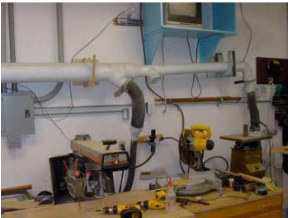
Figure 5: Is to the right of figure 4. I reduced the branch to 4" at this point. I think was a mistake. There are two blast gates here. One dedicated to the radial arm saw. The other goes to a flex hose and goes to a number of tools in that area.
